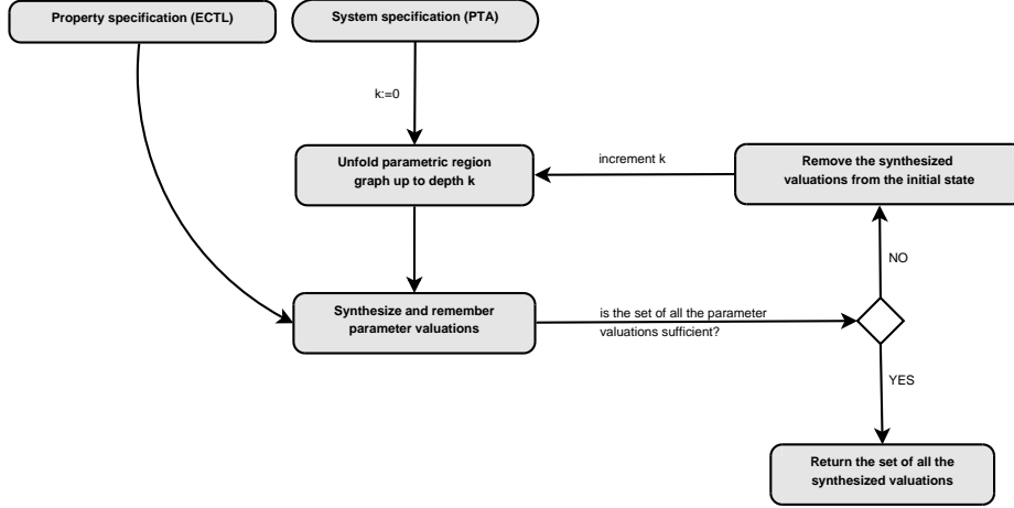
Fig. 1. Parametric Bounded Model Checking schema
