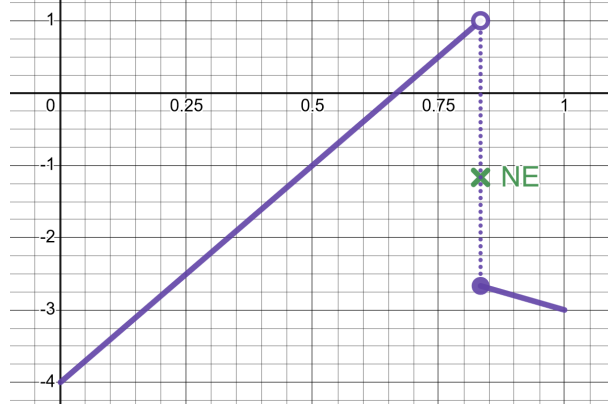
Fig. 6. V 's payoffs against best response for the Benaloh game in Figure 5b. The voter's payoff obtained by Nash equilibrium is shown for comparison
