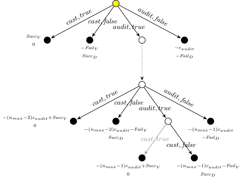
Fig. 4. Game tree for Benaloh challenge. V 's payoffs are in black, D 's payoffs in red
