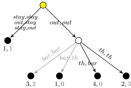
Fig. 3. Multi-step Battle of the Sexes. The initial state is filled with yellow, and terminal states with black. Transitions corresponding to dominated choices are shown in grey
