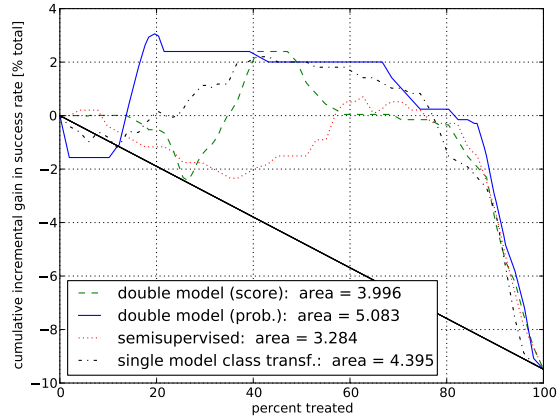
Figure 1. The uplift curve for the bone marrow trial data. The plot illustrates the difference between the incidence of chronic GVHD in the two arms of the study.
