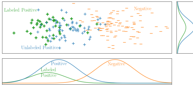
Fig. 2 Example of SAR PU and PGPU data. The labeled examples are a biased sample of the positive examples. The larger the probabilistic gap, the more likely a positive example is selected to be labeled. This means that positive examples which resemble negative examples more, are less likely to be labeled
